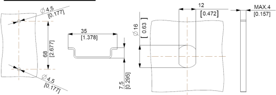
Drilling Templates
