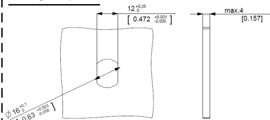
Drilling Templates
