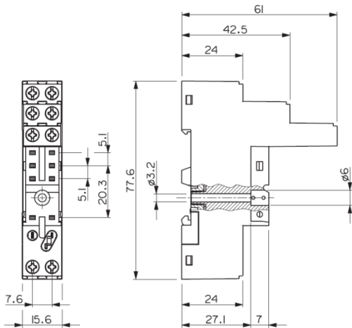
Dimensions Measures in (mm)
