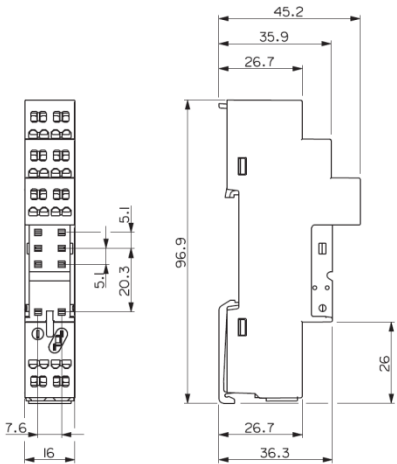
Dimensions Measures in (mm)
